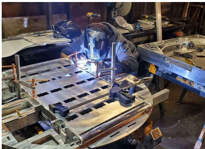
2022:01:12 17:25:04 - Welding Prototype
